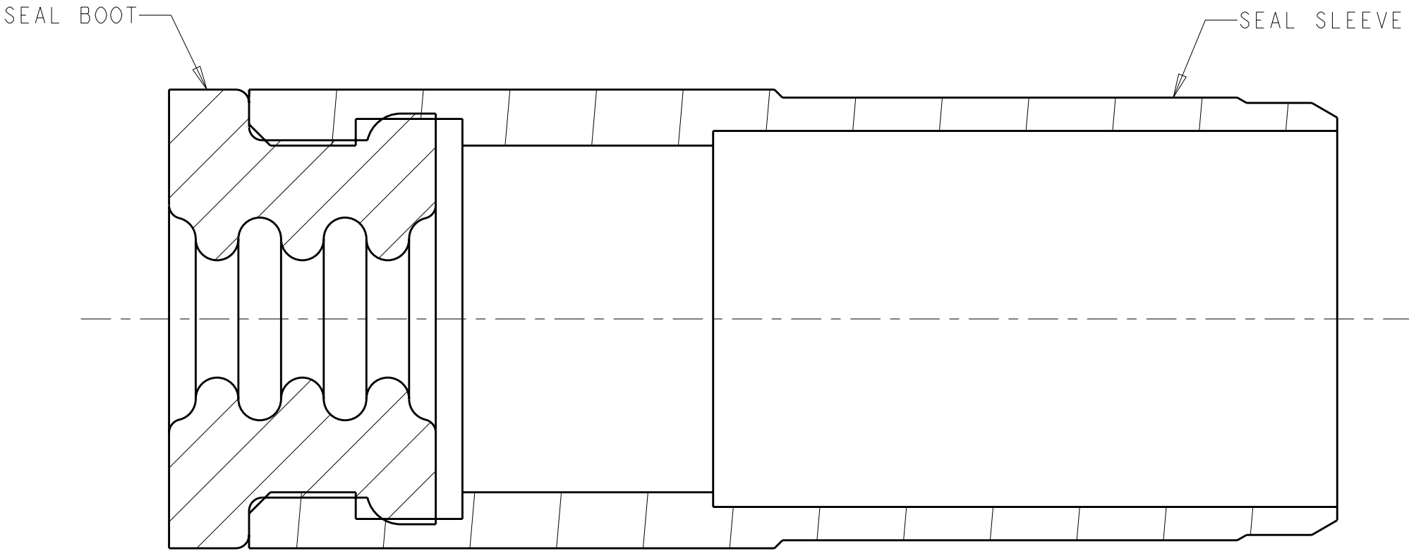
SECTION J-J
