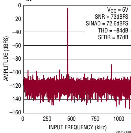
16k Point FFT, f_S = 2.5\text{Mps} f_{\text{IN}} = 497\text{kHz}
