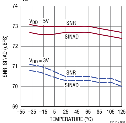
SNR, SINAD vs Temperature, f_{\text{IN}} = 497\text{kHz}
