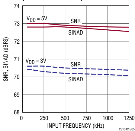
SNR, SINAD vs Input Frequency (100kHz to 1.2MHz)
