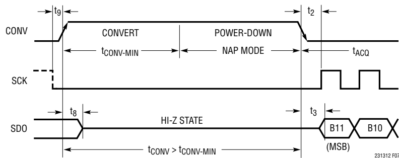
Figure 7. LTC2313-12 Nap Mode Power-Down Following Conversion for t_{\text{conv}} > t_{\text{conv-min}}
