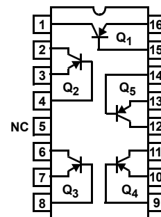
HFA3128 (16 LD SOIC) TOP VIEW
