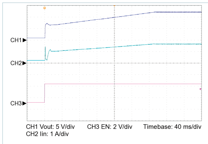
Figure 15 — Startup from EN, V_{IN} = 300\text{ V} , C_{OUT\_EXT} = 10000\text{ }\mu\text{F} , R_{LOAD} = 2.778\text{ }\Omega
