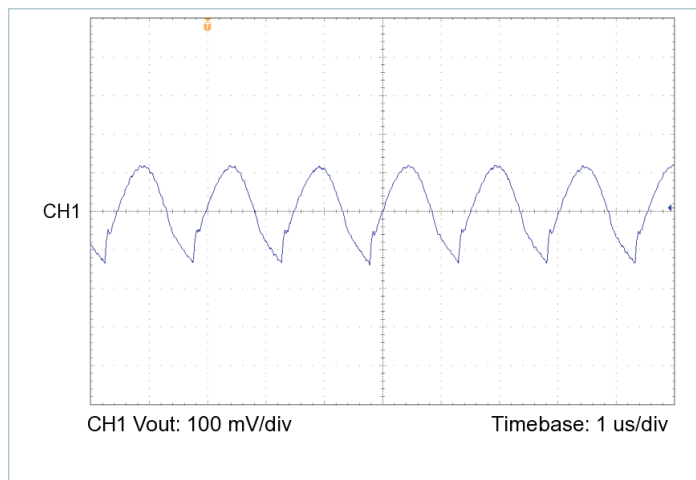
Figure 17 — Output voltage ripple, V_{IN} = 300\text{ V} , V_{OUT} = 12.0\text{ V} , C_{OUT\_EXT} = 1000\text{ }\mu\text{F} , R_{LOAD} = 2.778\text{ }\Omega
