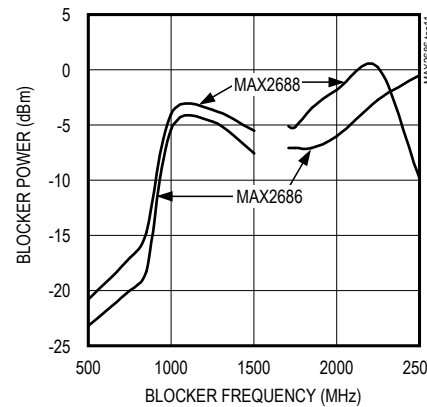
1dB GAIN DENSENSE vs. BLOCKER FREQUENCY
