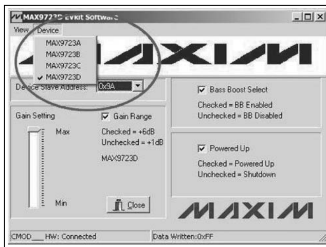
Figure 2. Device Selection and Slave Address
