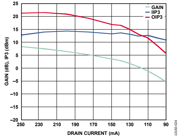
Figure 26. Gain and Input/Output IP3 vs. Drain Current, P_{IN} = -10 dBm/Tone, V_{CTL1}/V_{CTL2} = -1 V, RF = 71 GHz, Drain Current = ( I_{DD1}/I_{DD2} Fixed at 50 mA) + ( I_{DD3} to I_{DD6} Swept)
