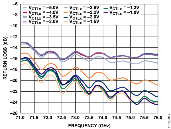
Figure 17. Input Return Loss vs. Frequency at Various Control Voltages
