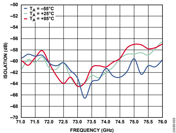
Figure 18. Reverse Isolation vs. Frequency at Various Temperatures, V_{CTL1}/V_{CTL2} = -5 V
