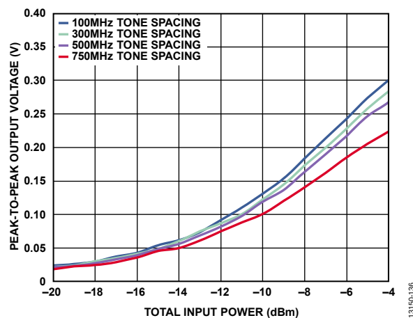
Figure 36. Envelope Detector Peak-to-Peak Output Voltage vs. Total Input Power at Various Tone Spacings, RF = 76 GHz, V_{CTL1}/V_{CTL2} = -5 V, V_{DET} = 4 V with 150\ \Omega Load Impedance at ENV_{DET}
