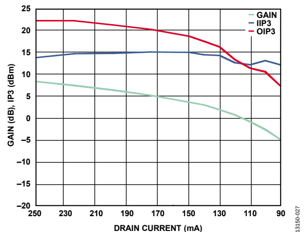
Figure 27. Gain and Input/Output IP3 vs. Drain Current, P_{IN} = -10 dBm/Tone, V_{CTL1}/V_{CTL2} = -1 V, RF = 73.5 GHz, Drain Current = ( I_{DD1}/I_{DD2} Fixed at 50 mA) + ( I_{DD3} to I_{DD6} Swept)
