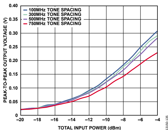
Figure 35. Envelope Detector Peak-to-Peak Output Voltage vs. Total Input Power at Various Tone Spacings, RF = 73.5 GHz, V_{CTL1}/V_{CTL2} = -5 V, V_{DET} = 4 V with 150\ \Omega Load Impedance at ENV_{DET}
