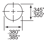
Mounting Hole
