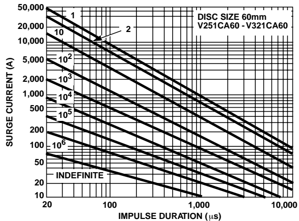
FIGURE 10. SURGE CURRENT RATING CURVES FOR V251CA60 - V321CA60
