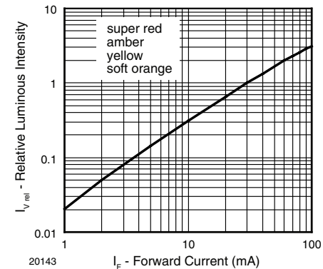
Figure 6. Relative Luminous Intensity vs. Forward Current
