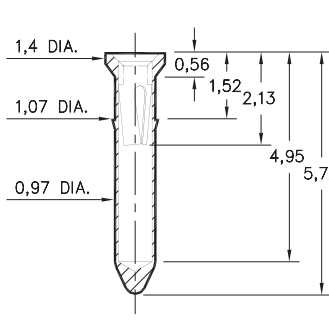
0579-0-15-XX-X1-XX-10-0 Press-fit in 1,02 mounting hole
