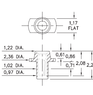
8874-0-15-XX-11-XX-10-0 Bottom entry Surface mount
