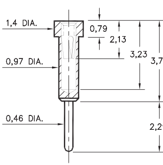
9407-0-15-XX-11-XX-10-0 Solder mount in 1,02 min. mounting hole
