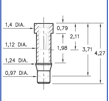
0613-0-15-XX-21-XX-10-0 Press-fit in 1,19 mounting hole
