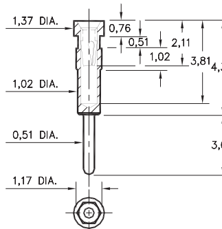
9462-0-15-XX-21-XX-04-0 Hex press-fit in 1,09 plated thru hole
