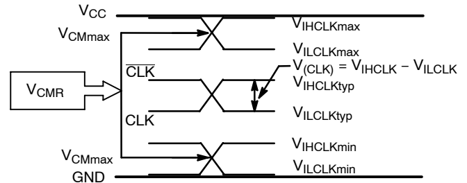
Figure 13. V_{CM} Diagram
