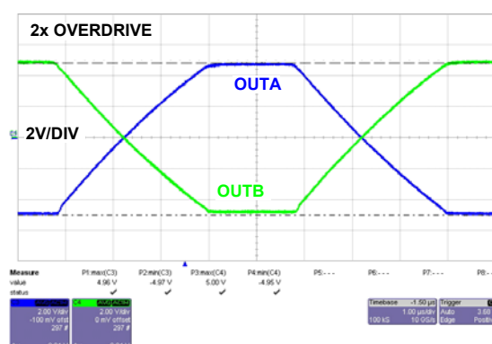
FIGURE 30. OVERDRIVE RECOVERY
