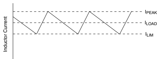
Figure 30 - Valley Current Limit
