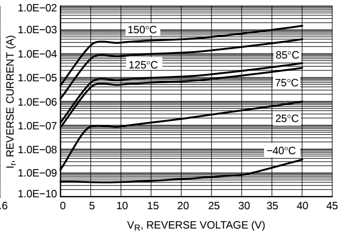
Figure 2. Leakage Current
