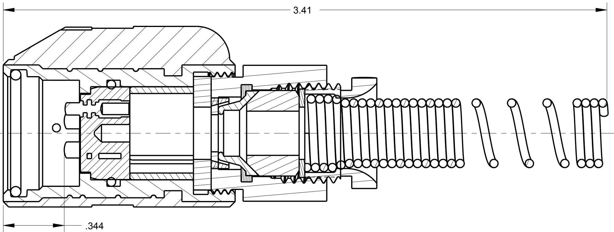
SECTION Z-Z
