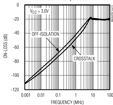
FREQUENCY RESPONSE OFF-ISOLATION, CROSSTALK
