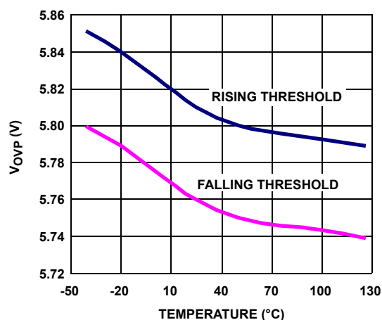
FIGURE 13. INPUT OVERVOLTAGE PROTECTION THRESHOLDS vs TEMPERATURE
