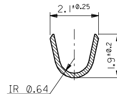
SECT. C-C
