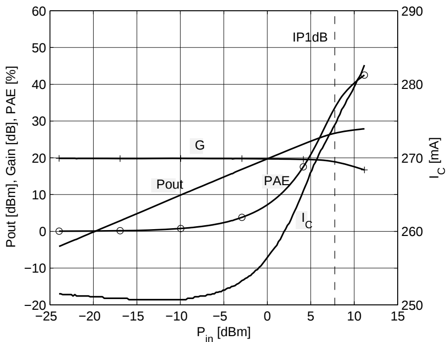
Figure 7-20 P_{out} , Gain, I_C , PAE vs. P_{in} at V_{CE} = 5\text{ V} , I_{Cq} = 250\text{ mA} , f = 0.9\text{ GHz} , Z_l = Z_{opt}
