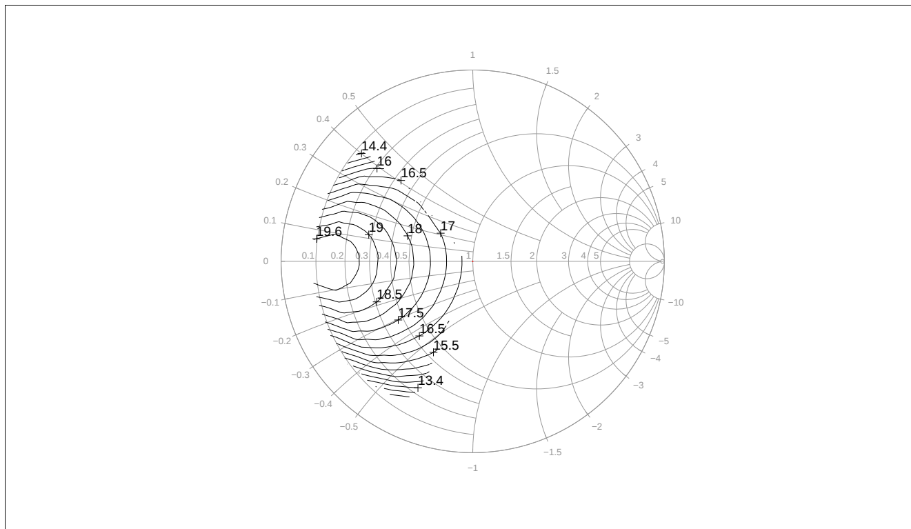
Figure 7-18 Load Pull Contour Gain G [dB] at V_{CE} = 5\text{ V} , I_C = 250\text{ mA} , f = 0.9\text{ GHz} , Z_I = Z_{opt}
