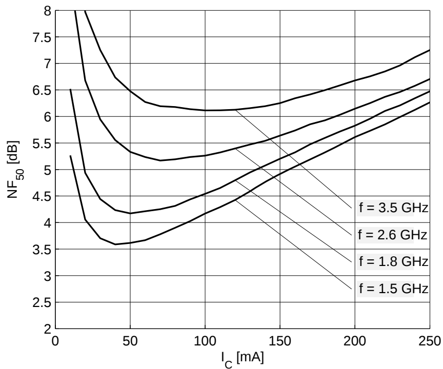
Figure 7-15 Noise Figure NF_{50} vs. I_C at V_{CE} = 5 V, Z_S = 50 \Omega , f = Parameter
