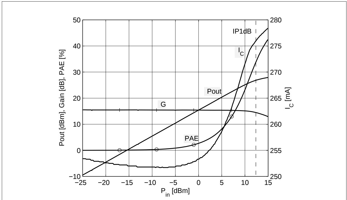
Figure 7-21 P_{out} , Gain, I_C , PAE vs. P_{in} at V_{CE} = 5 V, I_{Cq} = 250 mA, f = 2.6 GHz, Z_L = Z_{opt}
