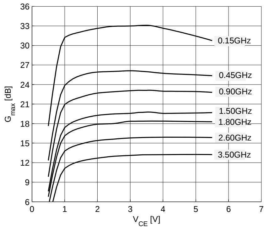
Figure 7-9 Maximum Power Gain G_{\max} vs. V_{CE} at I_C = 250 mA, f = Parameter
