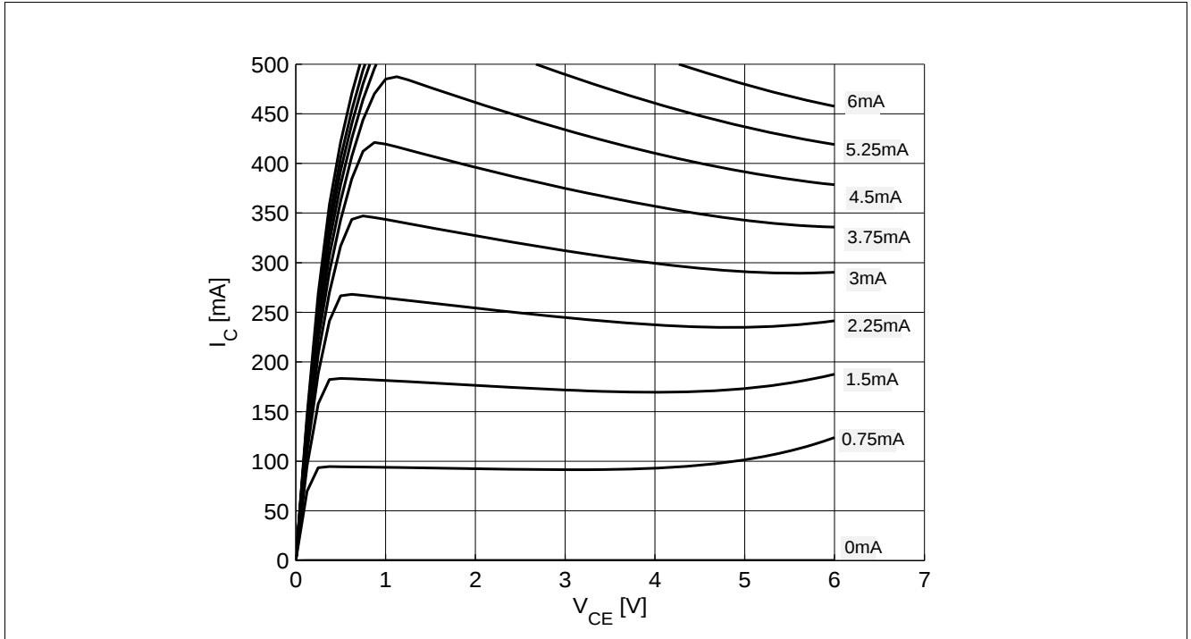
Figure 7-2 Collector Current I_C vs. V_{CE} , I_B = Parameter
