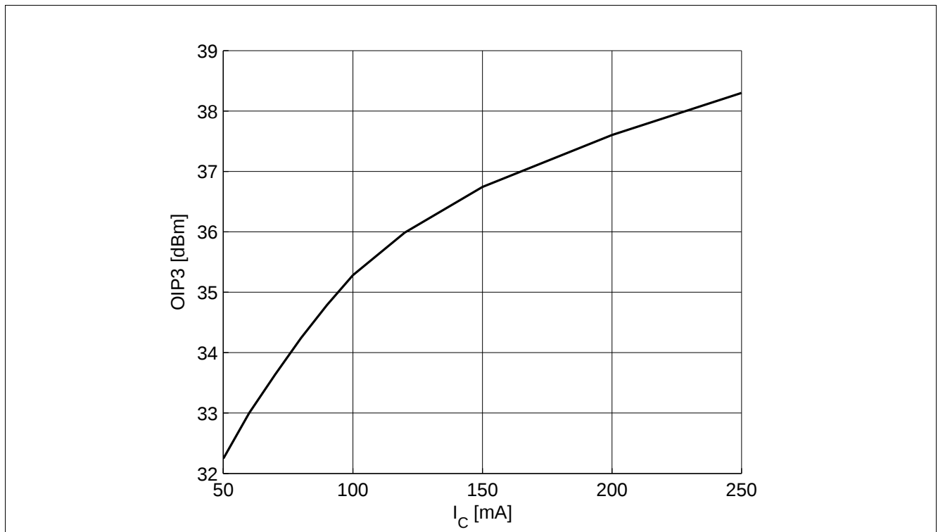
Figure 7-22 OIP3 vs. I_C at V_{CE} = 5 V, f = 0.9 GHz, Z_L = Z_{Lopt}
