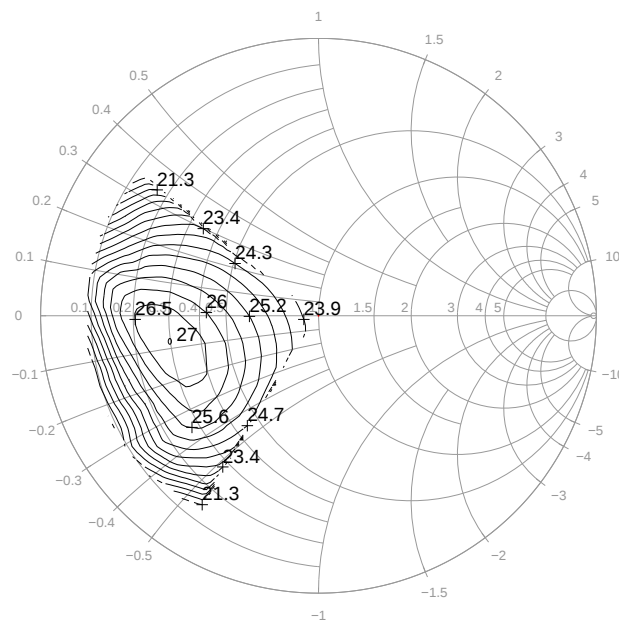
Figure 7-16 Load Pull Contour OP_{1dB} [dBm] at V_{CE} = 5 V, I_C = 250 mA, f = 0.9 GHz, Z_I = Z_{opt}
