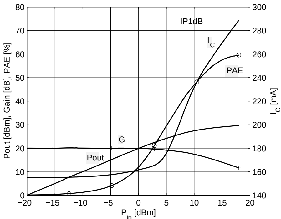
Figure 7-19 P_{out} , Gain, I_C , PAE vs. P_{in} at V_{CE} = 5\text{ V} , I_{Cq} = 155\text{ mA} , f = 0.9\text{ GHz} , Z_l = Z_{opt}
