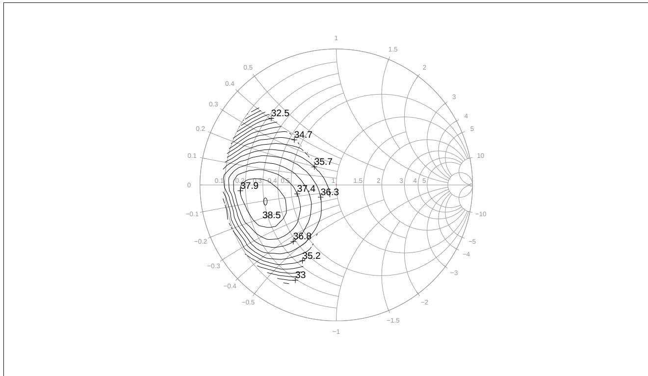
Figure 7-17 Load Pull Contour OIP3 [dBm] at V_{CE} = 5\text{ V} , I_C = 250\text{ mA} , f = 0.9\text{ GHz} , Z_I = Z_{opt}
