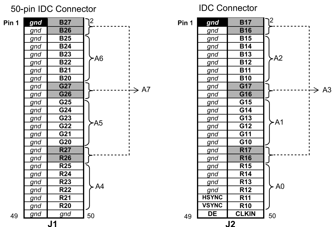
Figure 4. Mapping for New Mode (Transmitter Board)
