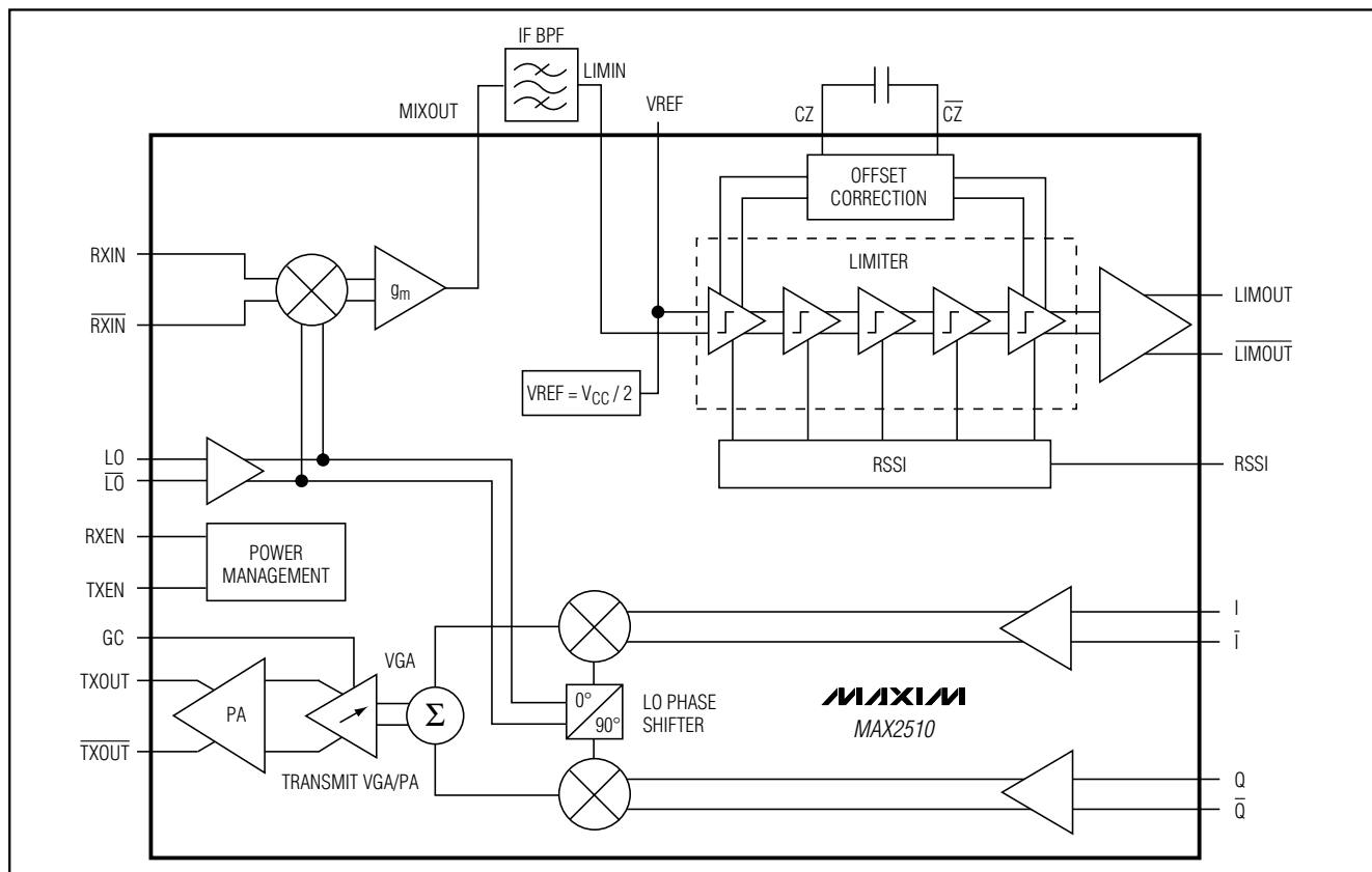
Figure 1. Functional Diagram
