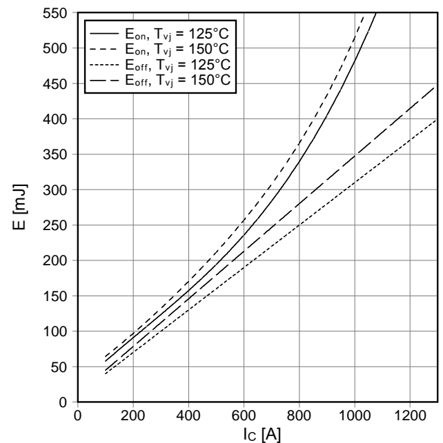
Schaltverluste IGBT-Wechselr. (typisch) switching losses IGBT-inverter (typical) E_{on} = f(I_C) , E_{off} = f(I_C) V_{GE} = \pm 15\text{ V} , R_{Gon} = 1\ \Omega , R_{Goff} = 2.7\ \Omega , V_{CE} = 900\text{ V}
