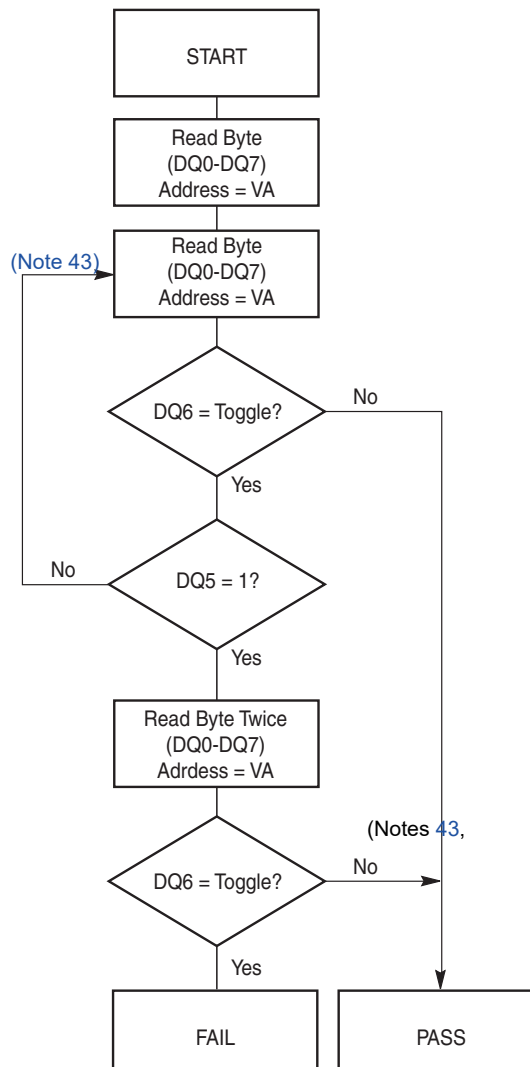
Figure 8. Toggle Bit Algorithm
