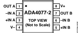
Figure 5. Pin Configuration, 8-Lead SOIC_N (R Suffix)
