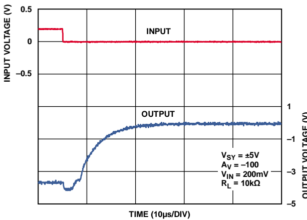
Figure 44. Negative Overload Recovery
