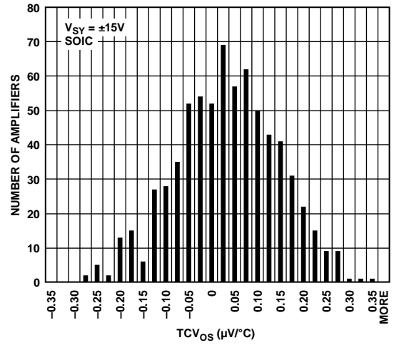
Figure 15. TCV_{OS} , SOIC
