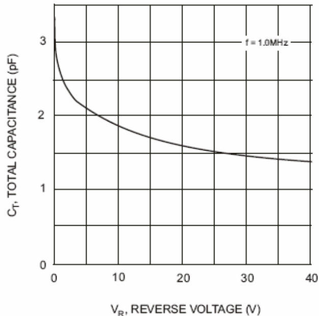
Fig. 3 Typical Capacitance
