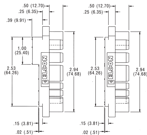
Float-Mount Part Number 6648167-1
