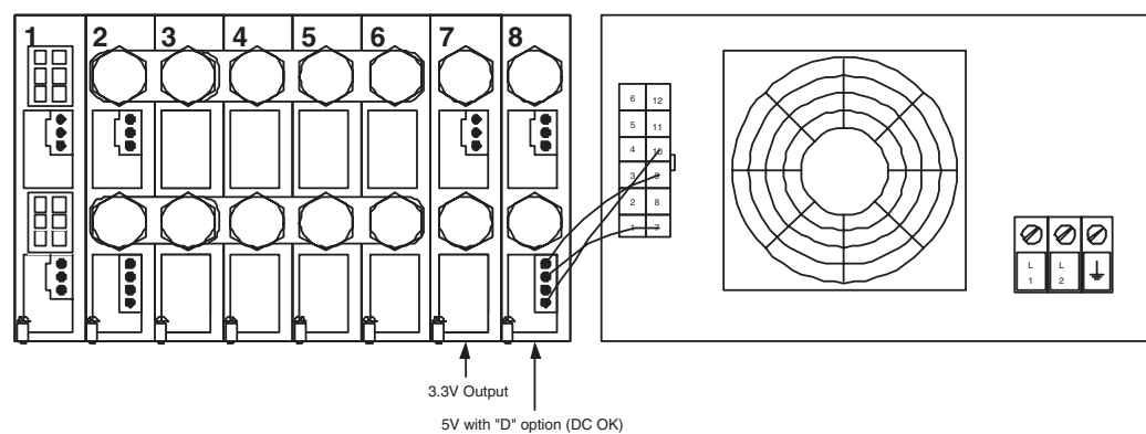
Figure 17 Output sequencing wire interconnect
