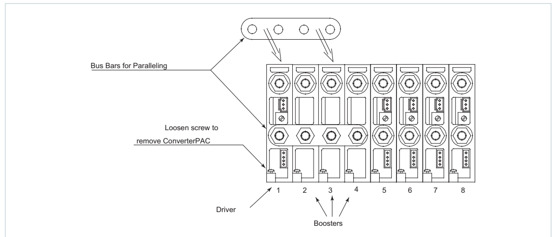
Figure 2 Paralleling ConverterPACs
