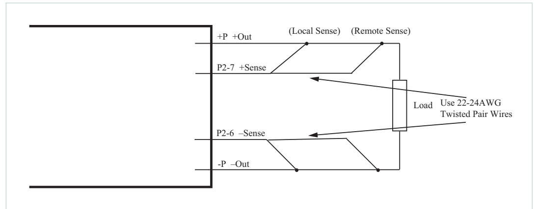
Figure 10 Sense Leads
