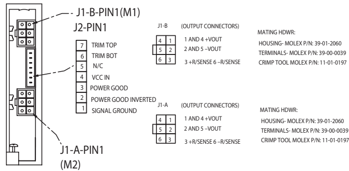
DUALQPAC - COMPONENT SIDE VIEW
