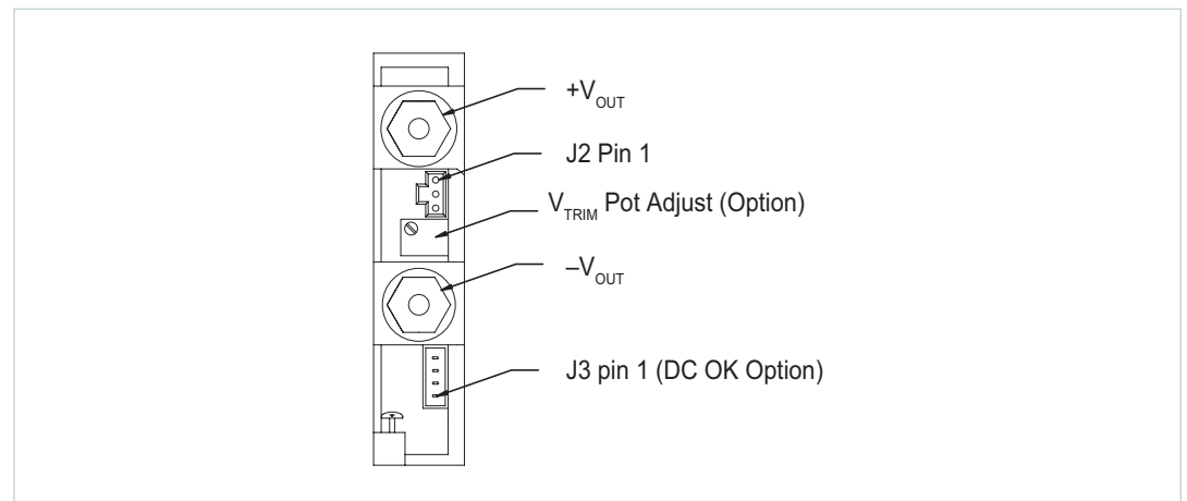
Figure 15 QPAC pinout
