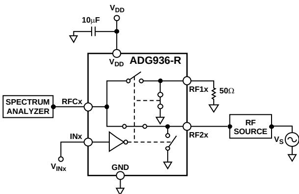
Figure 26. P_{-1\text{ dB}}
