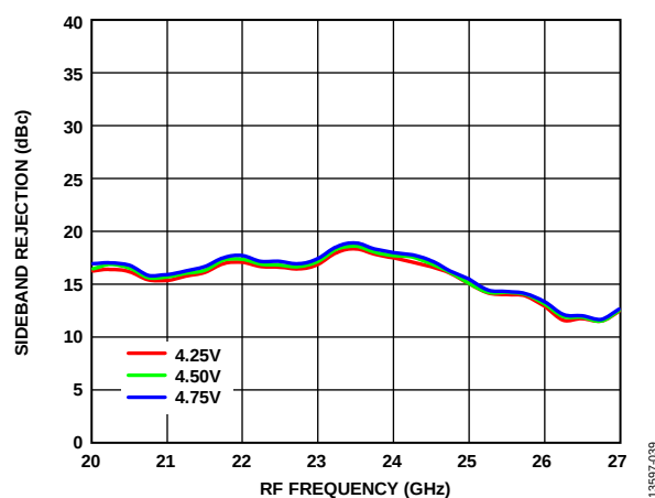
Figure 39. Sideband Rejection vs. RF Frequency over VDD1, LO Power = 4 dBm, T_A = 25^\circ\text{C}
