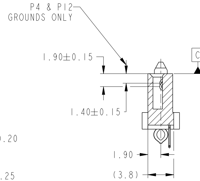
SECTION X-X
