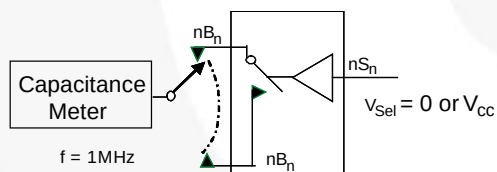
Figure 17. Channel Off Capacitance
