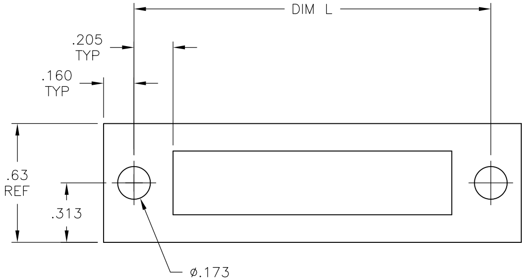
RECOMMENDED PANEL LAYOUT
