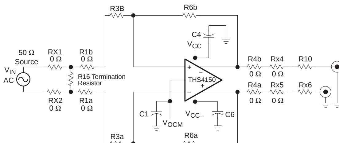
Figure 1–3. Fully-Differential In/Fully-Differential Out, Without Transformer
