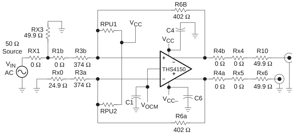
Figure 1–5. VICR Level Shifter
