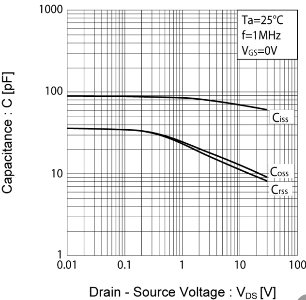
Fig.14 Typical Capacitance vs. Drain - Source Voltage
