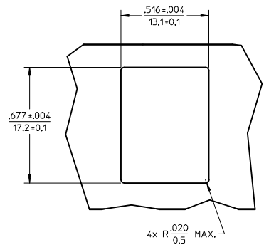
RECOMMENDED MOUNTING PATTERN SCALE 2.5:1 FOR .063 THICK PANEL 1.6
