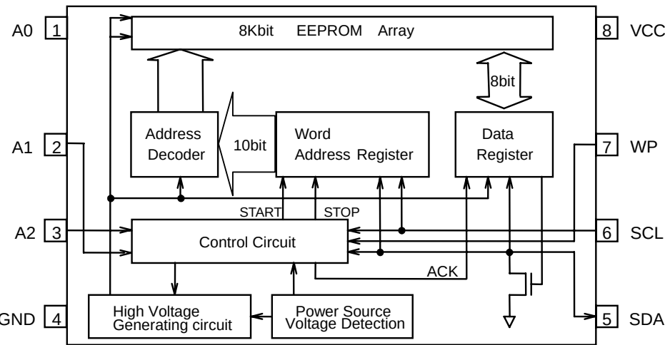
Figure 3. Block Diagram
