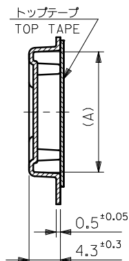
SECT. V-V
