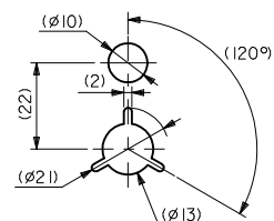
DETAIL "E"
