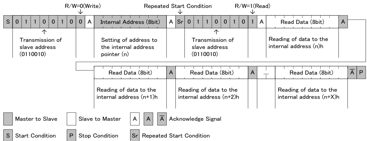
Fig 11-5 I2C-Bus Data Transmission Read Format
