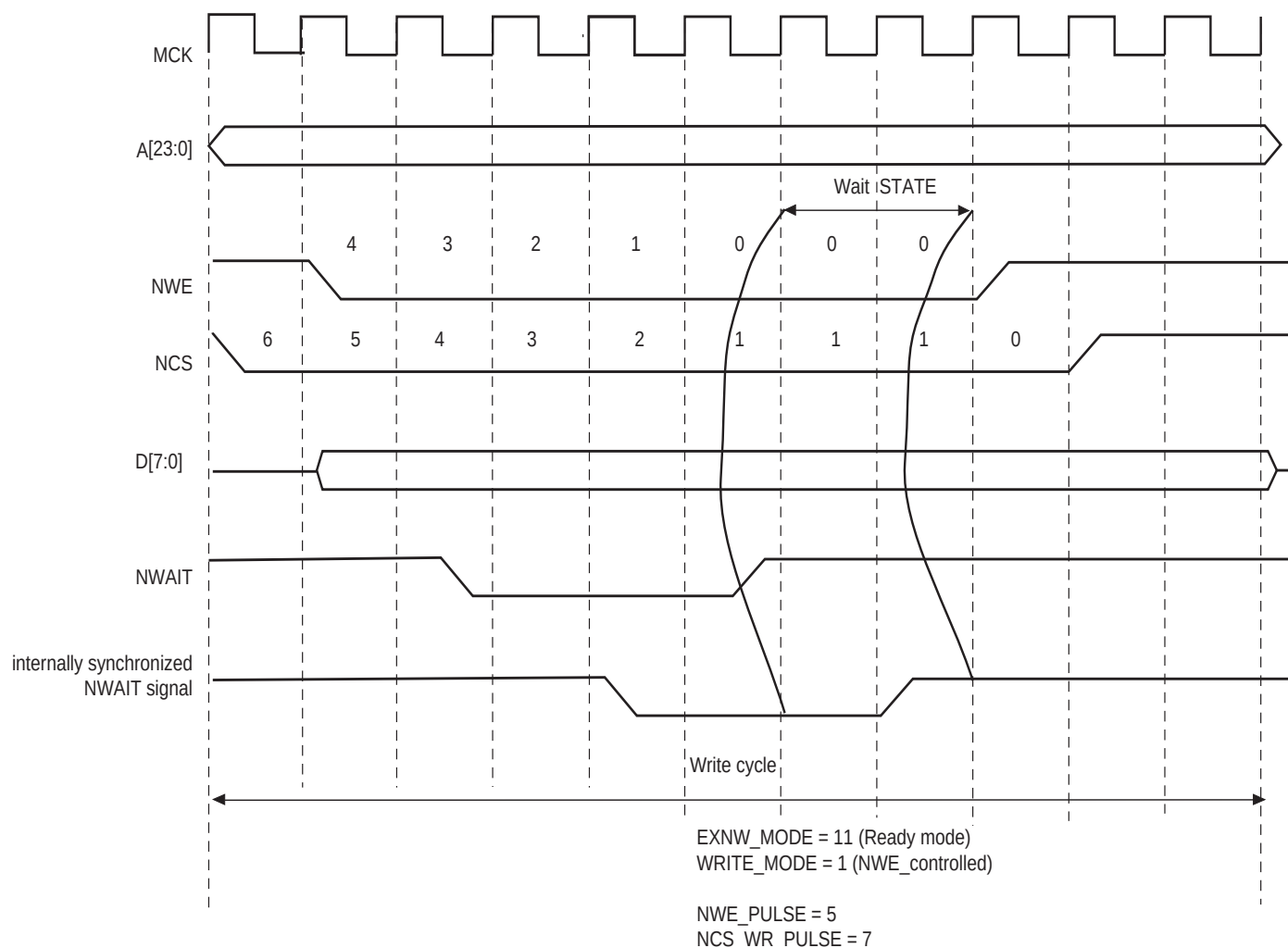
Figure 23-25. NWAIT Assertion in Write Access: Ready Mode ( \text{EXNW\_MODE} = 11 )
