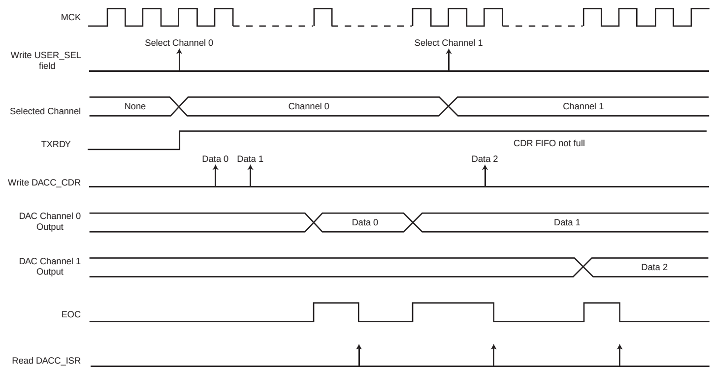
Figure 40-2. Conversion Sequence
