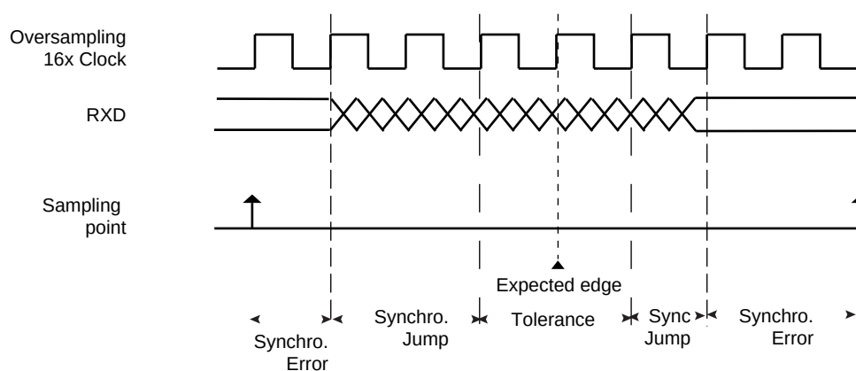
Figure 33-11. Bit Resynchronization
