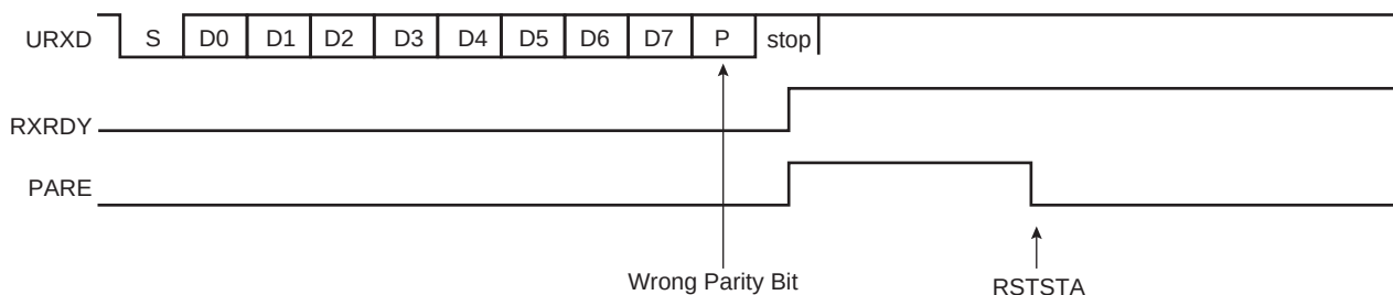
Figure 32-7. Parity Error
