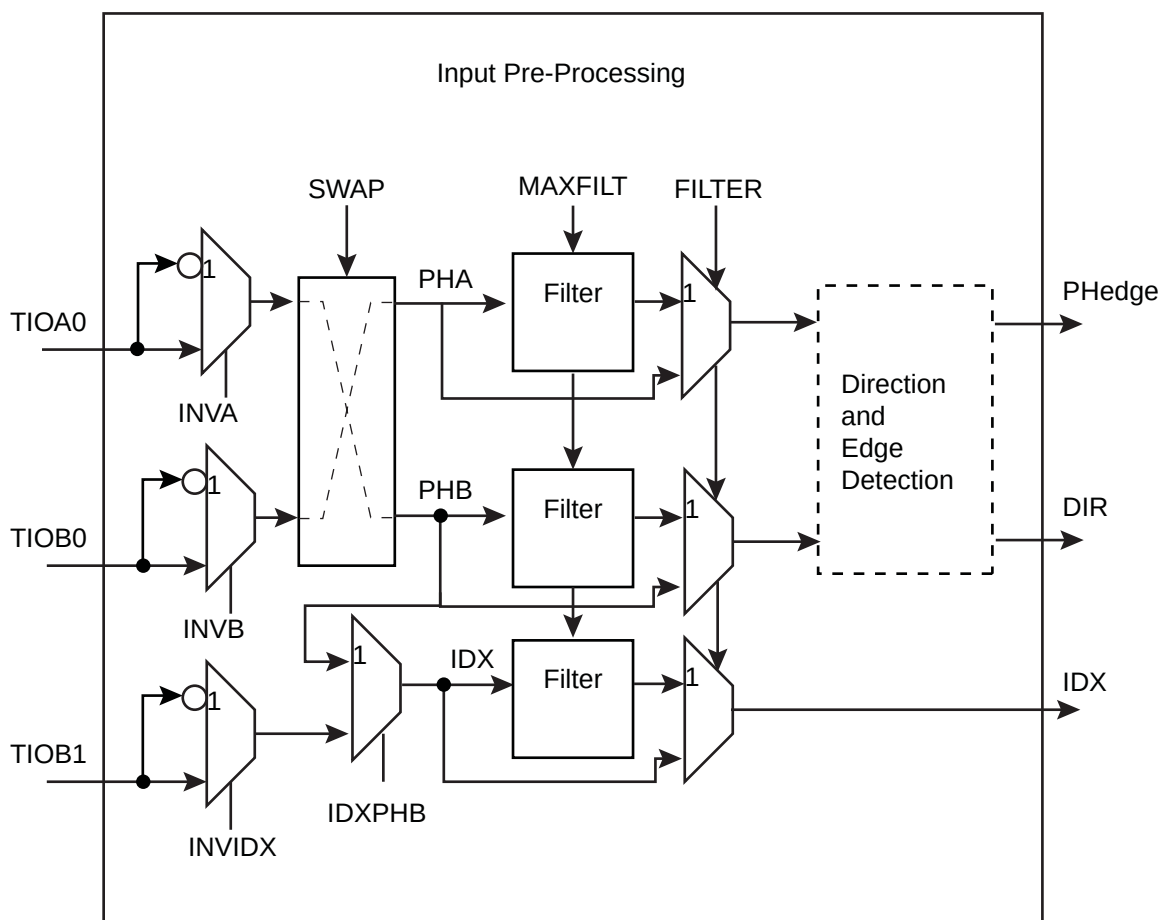
Figure 34-16. Input Stage
