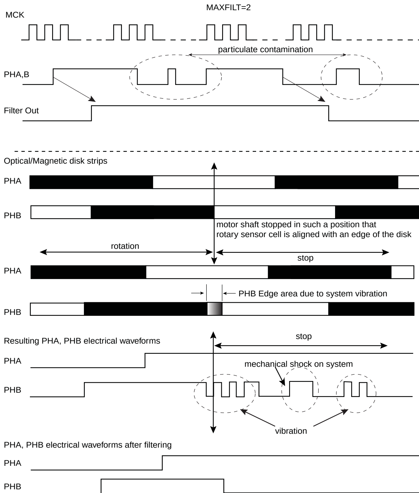
Figure 34-17. Filtering Examples
