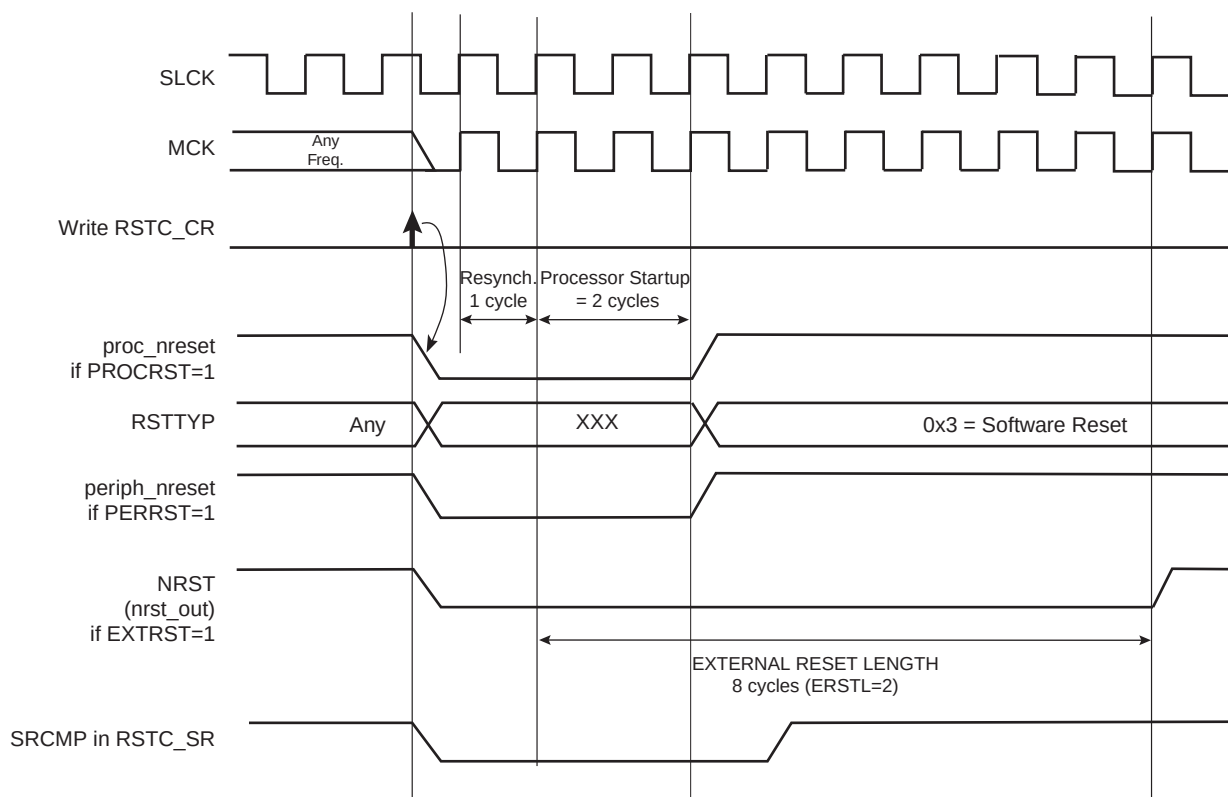
Figure 12-5. Software Reset
