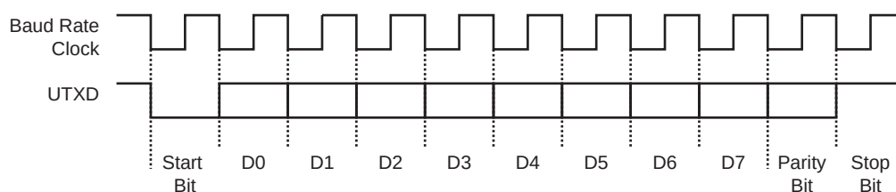
Figure 32-9. Character Transmission
