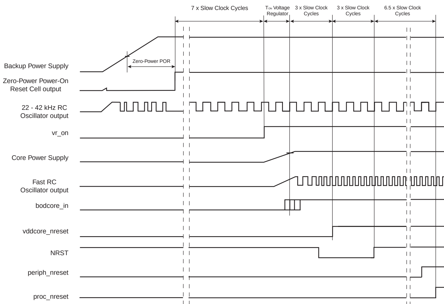
Figure 16-3. Raising the VDDIO Power Supply
