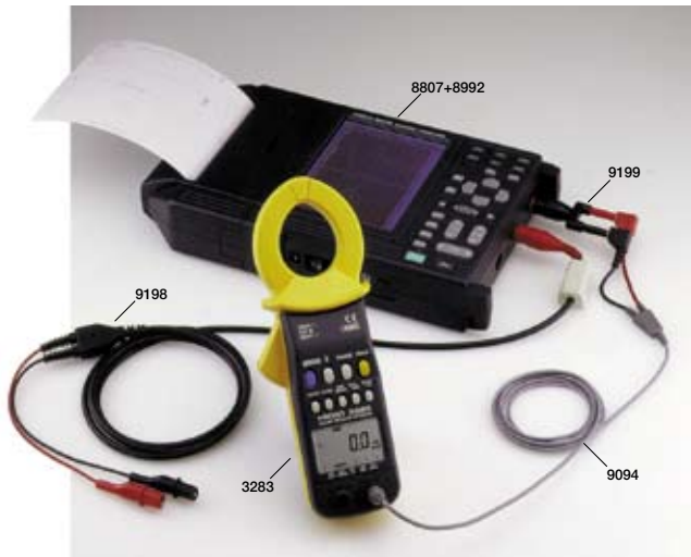
For long-term monitoring, use the AC ADAPTER 9418-15 for the MEMORY HICORDER 8807-01 and the AC ADAPTER 9445-02/-03 for the CLAMP ON LEAK HITESTER 3283
