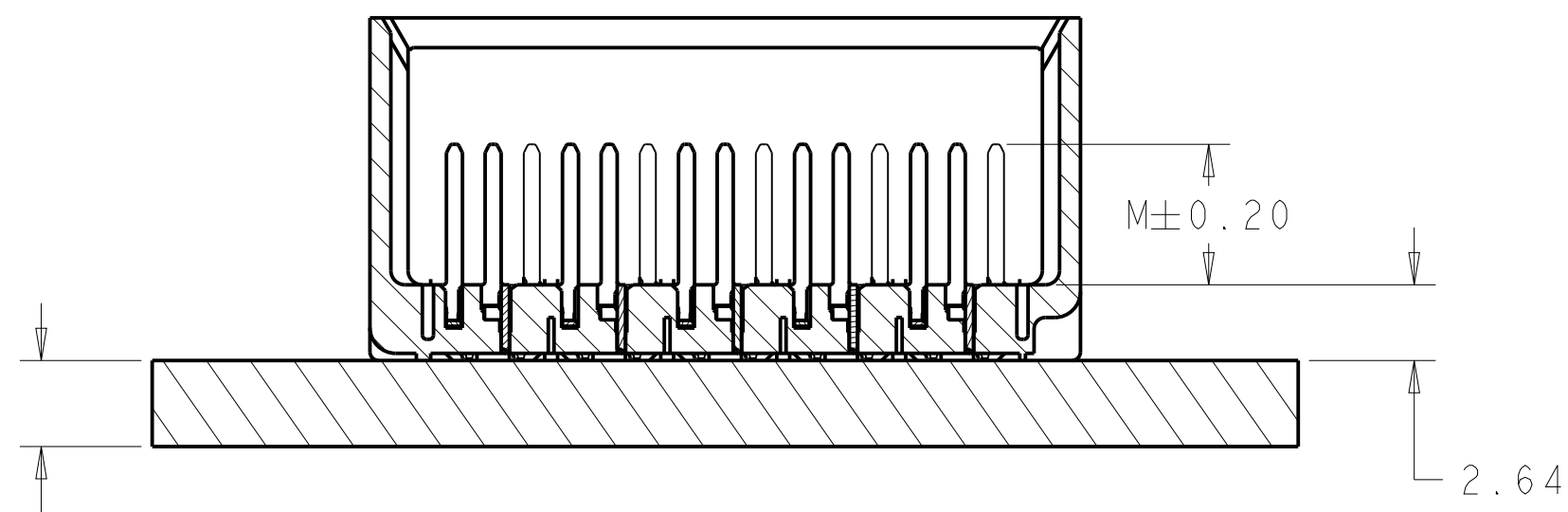
SECTION Z-Z
