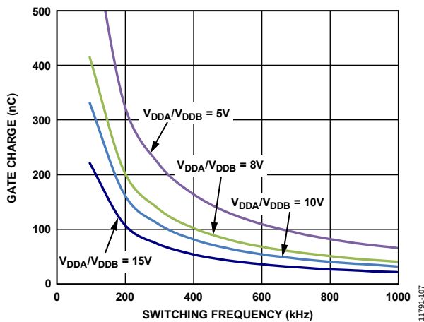
Figure 7. Typical ADuM3224 Maximum Load vs. Switching Frequency ( R_G = 1 \Omega )
